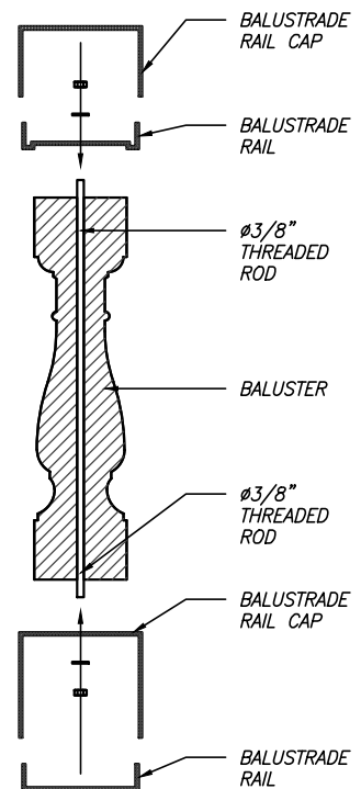
TYPICAL BALUSTER AND RAIL ASSEMBLY
